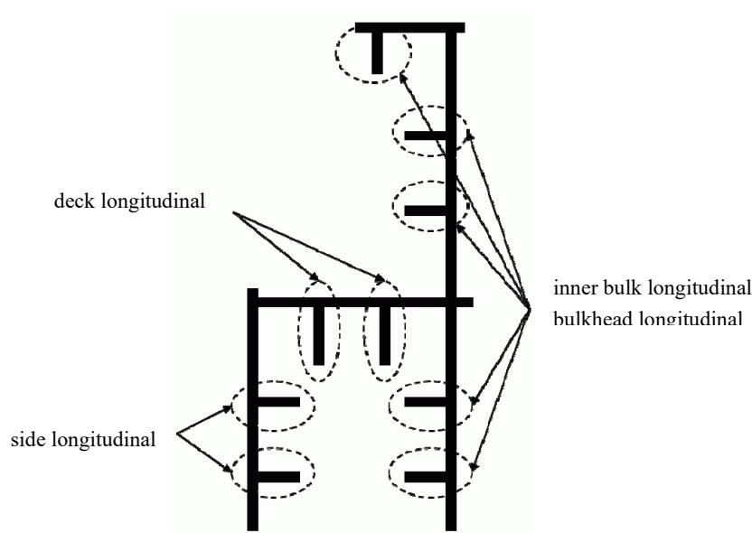
Fig. 2.10.1.1 Upper flange longitudinal structural members
