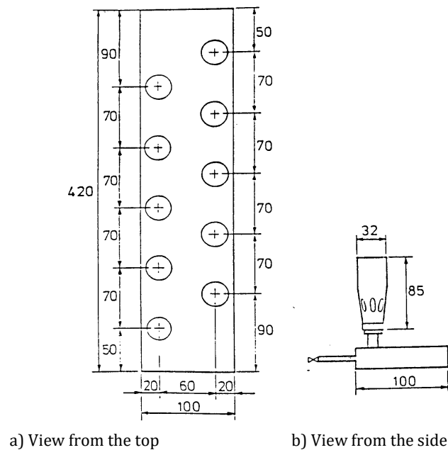
Figure 1. Burners array
