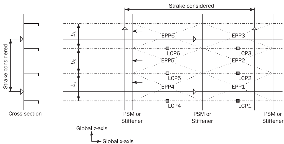
Figure 19 : Load calculation point for transverse framing
