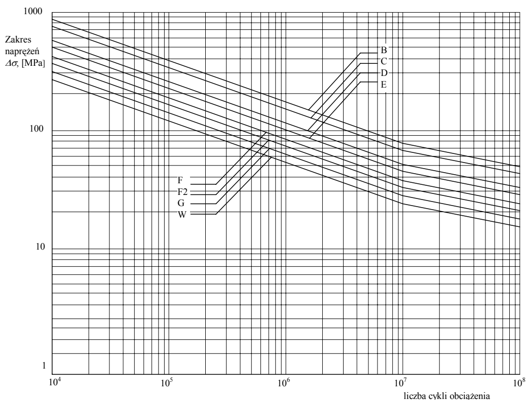
Fig. 2.4.3 S-N curve (s)
