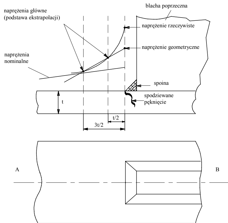
Fig. 4.2.4.1 Definition of hot-spot stresses
