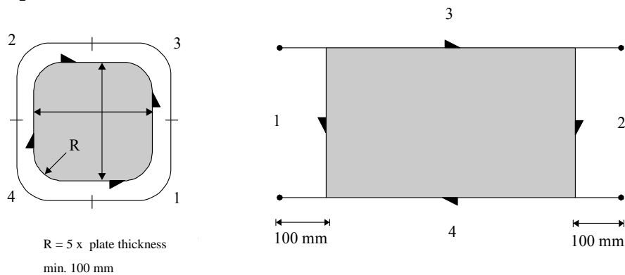
Fig. 6.2 Welding sequence for inserts
