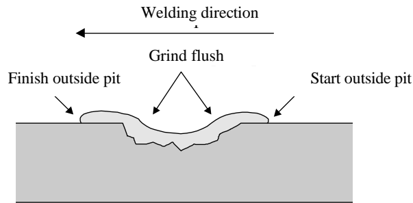
Fig. 6.7 Welding of pits
