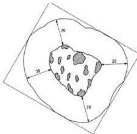
Fig. 4.2.2 (b) – Determination of the area influenced by clustered discontinuities (Re. EN 10163-1:2004+AC:2007 E)
