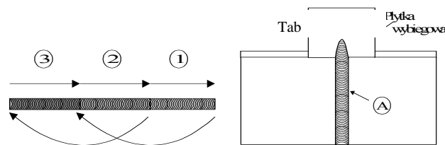
Fig. 6.8 a Step back technique
