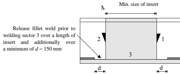
Fig. 6.4 Welding sequence for inserts of stiffeners
