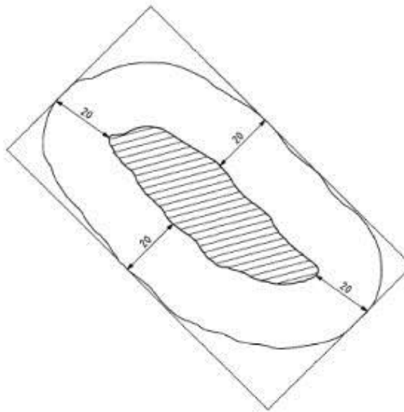
Fig. 4.2.2 (a) – Determination of the area influenced by an isolated discontinuity (Re. EN 10163-1:2004+AC:2007 E)
