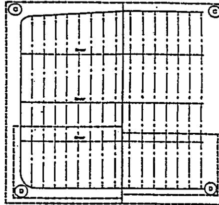
Oil tanker Typical transverse bulkhead
