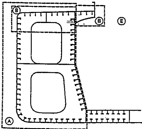
Ore/oil ship Typical transverse section close-up sur-
