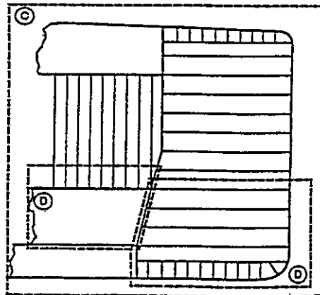
Ore/oil ship Typical transverse bulkhead
